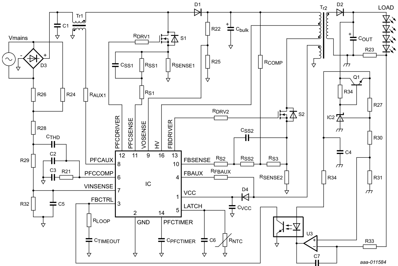
Fig 16. SSL8516T typical application diagram
